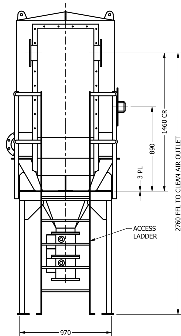
FILTER SIDE
