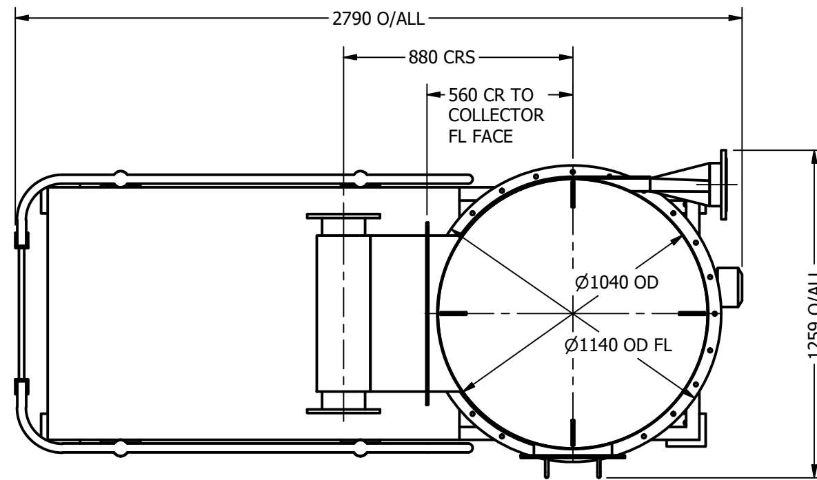
PLAN VIEW
